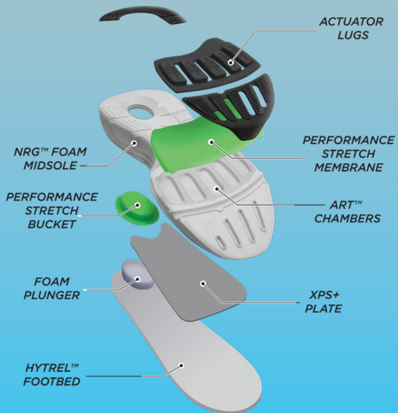
Exploded View of Sole Construction
